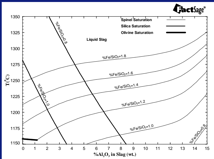
Above: Impact of Al_2O_3 on the Noranda Reactor slag temperature (FactSage)
