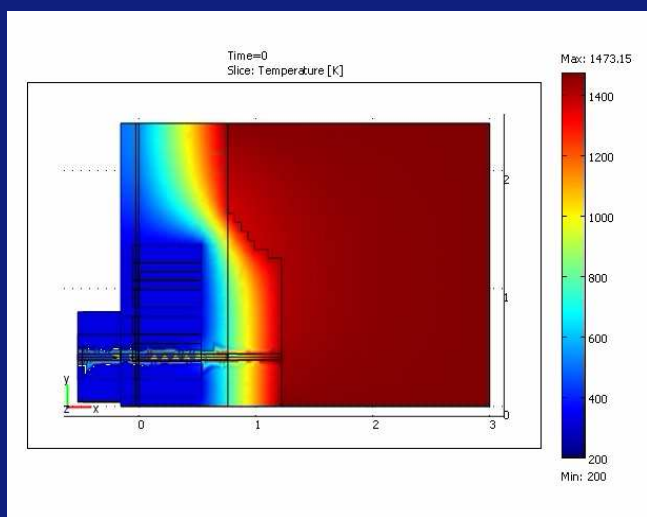
Finite Element study on a tap hole of an electric furnace
