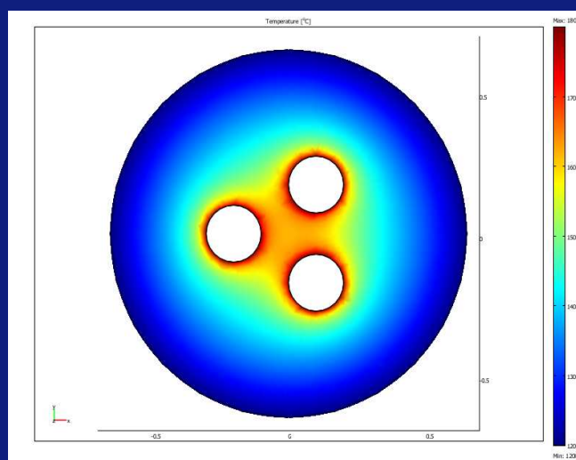
Temperature profile in the slag phase of AC submerged furnace
